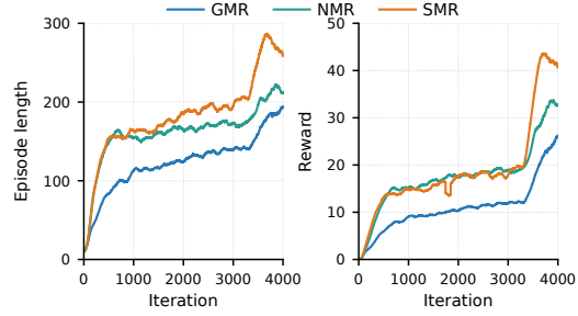
Figure 5: MimicLite training with different motion references. SMR achieves longer episodes and higher rewards by 4,000 iterations.
