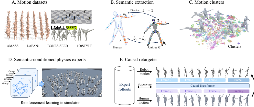
Figure 1: Overview of SMR. (A–C) Human motions from multiple datasets are converted into robot-aware task-space semantics and grouped for expert training. (D) Physics experts track these targets directly in simulation. (E) Accepted expert state rollouts supervise a single strictly causal transformer that generates robot motion references from current and past human observations.
