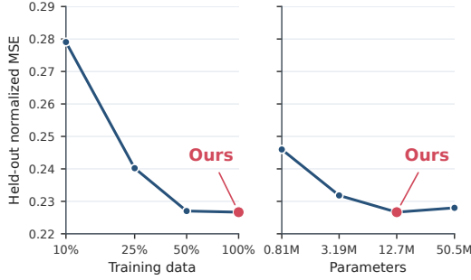
Figure 4: Data and model scaling. Gains diminish beyond 50% training data, while the 12.7M model achieves the lowest held-out error.
